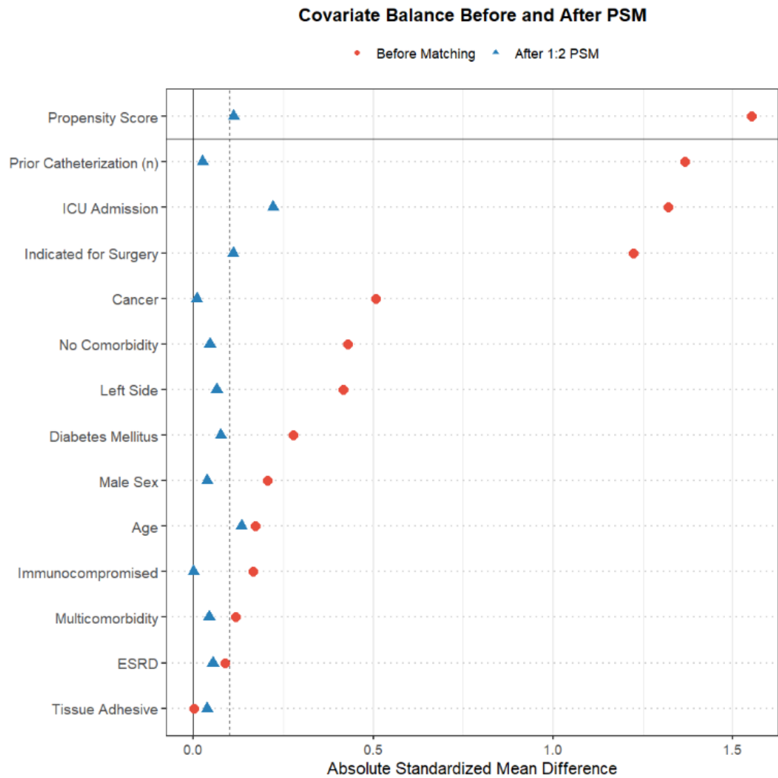
Supplementary Fig. 1. Love plot of propensity score matching. PSM, propensity score matching; ESRD, end-stage renal disease.
